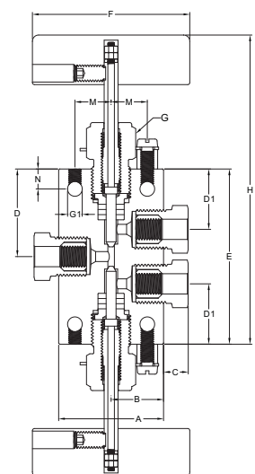
3-way/2 stem manifold
