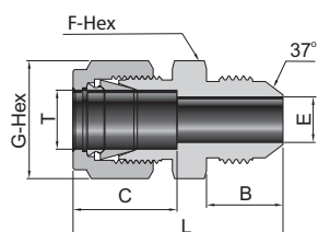
Fractional Tube
