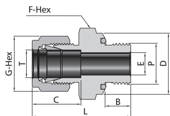
Fractional Tube
