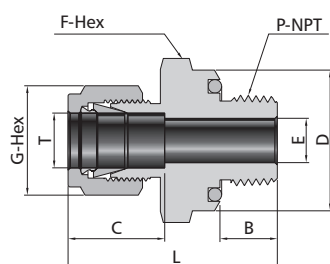
Fractional Tube
